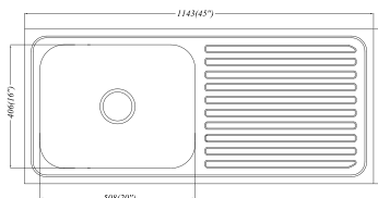
DRAINER WASTE
