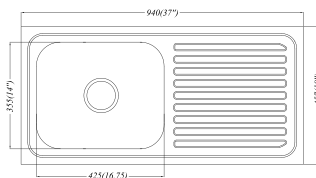
DRAINER WASTE
