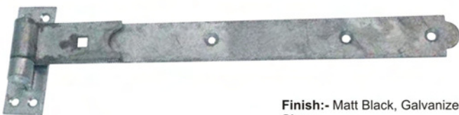
RA-IH-173 - Heavy Steel Hook & Band Hinge Straight
