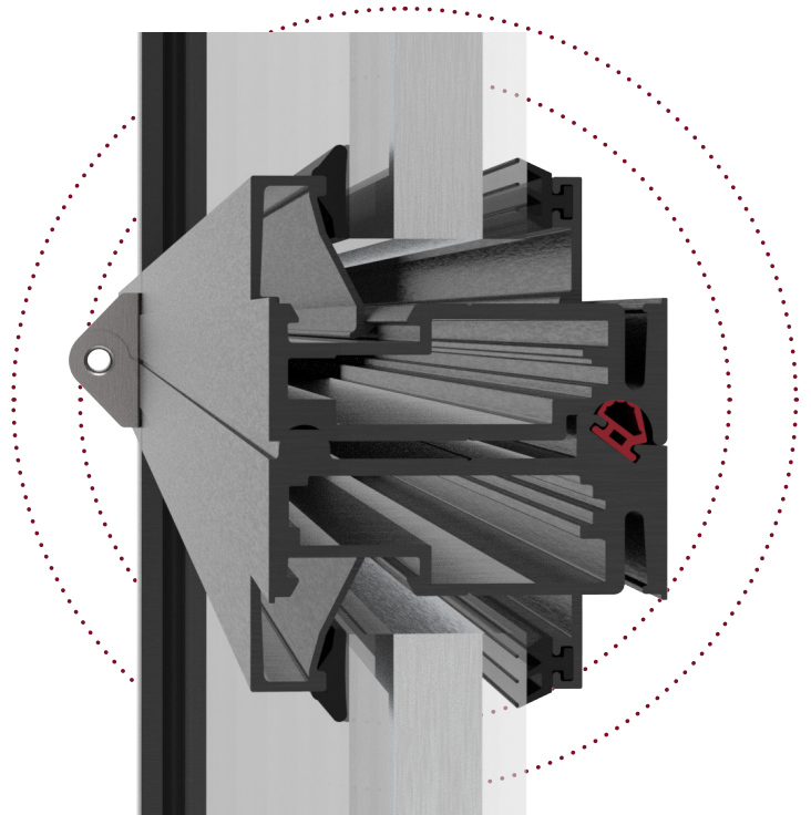
WindLyft S Cross Section
