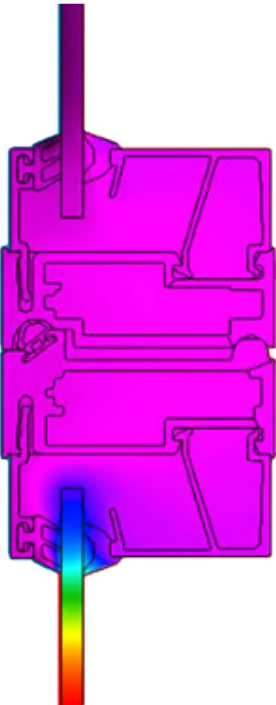
UNINSULATED GARAGE DOOR
