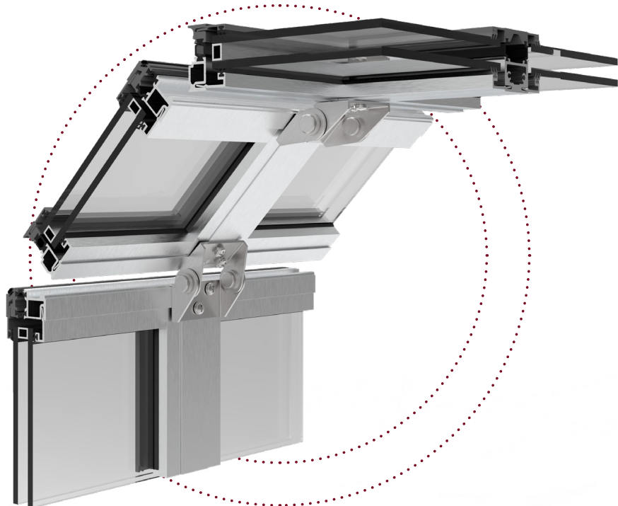
WINDLYFT HTP Cross Section
