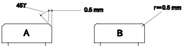
Figure 11. Épée: details of tip of point
