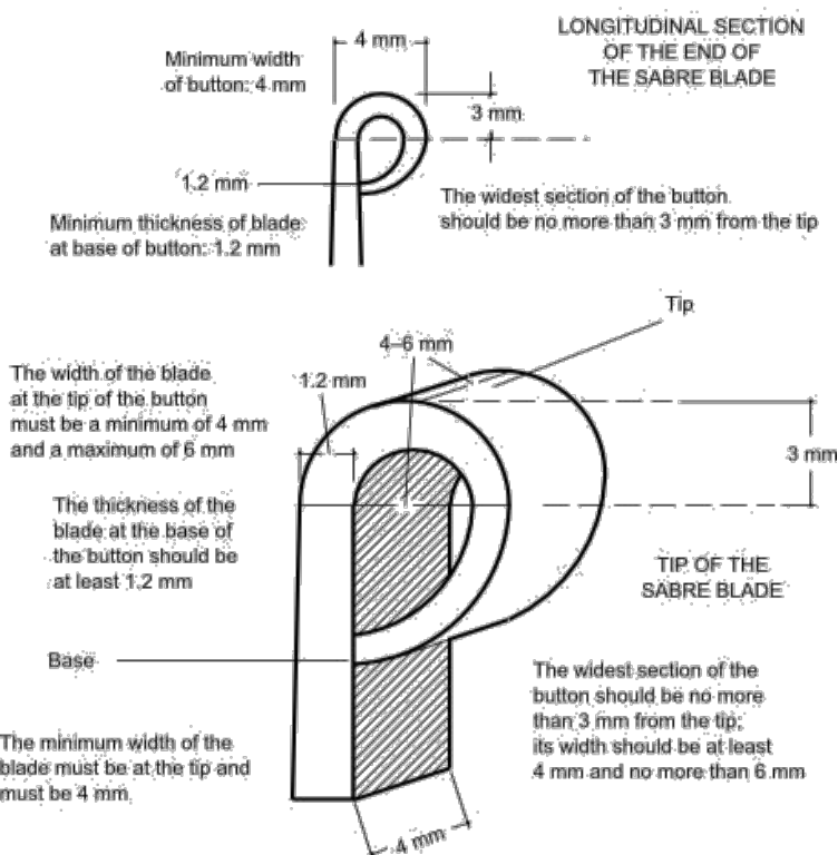
Figure 12. Sabre dimensions and flexibility
