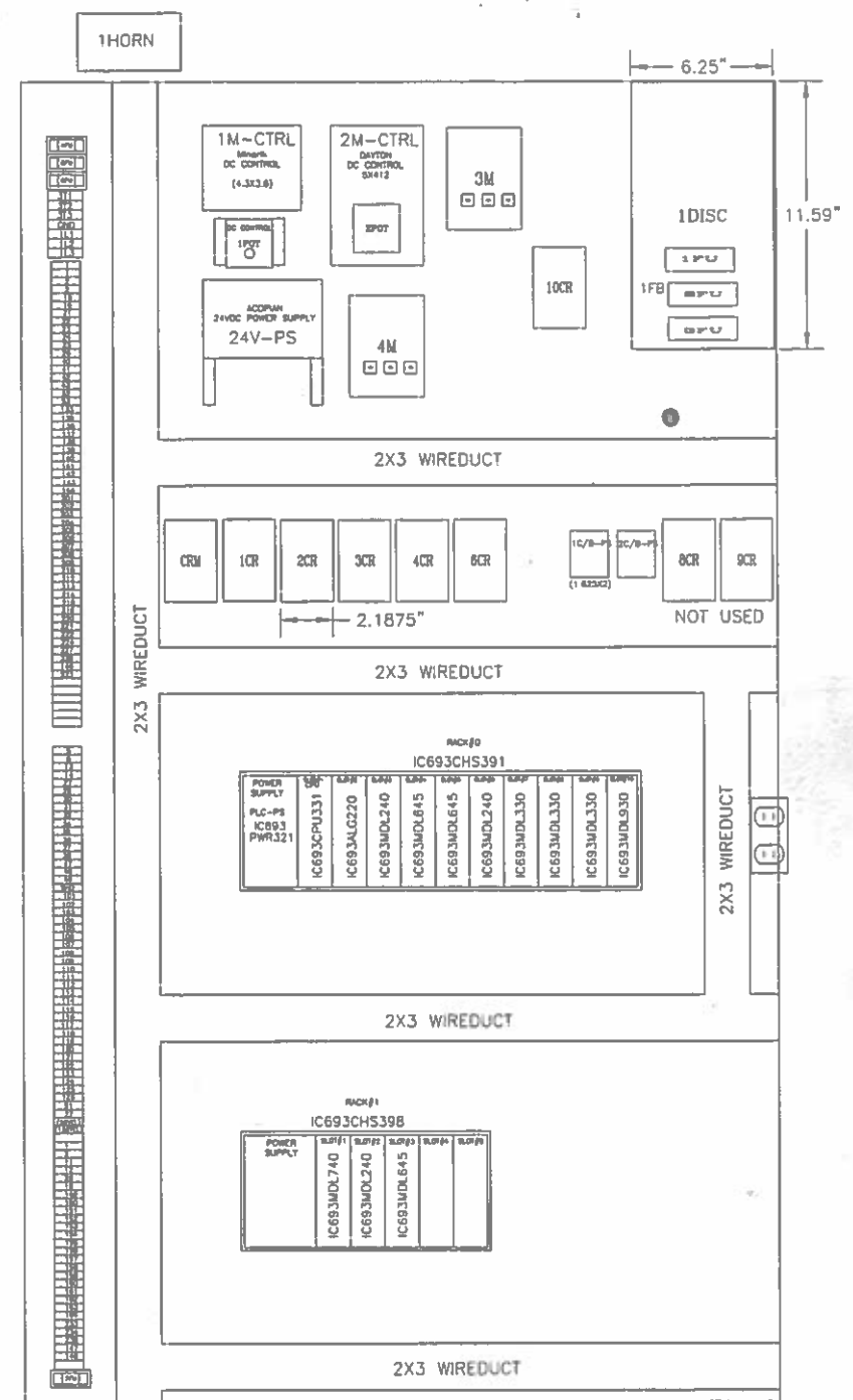
MAIN CONTROL PANEL ENCLOSURE #1 HOFFMAN ENCLOSURE A-60A83810LP PANEL A-60P36 (57X33)
