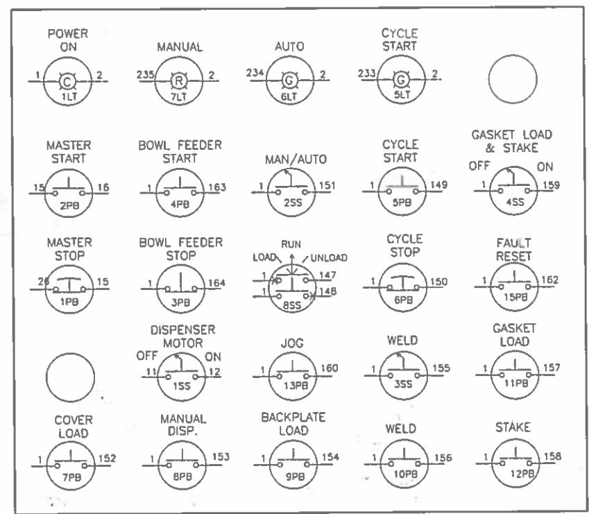
JB#11 OPERATOR'S PANEL 25 HOLE PUSH BUTTON BOX
