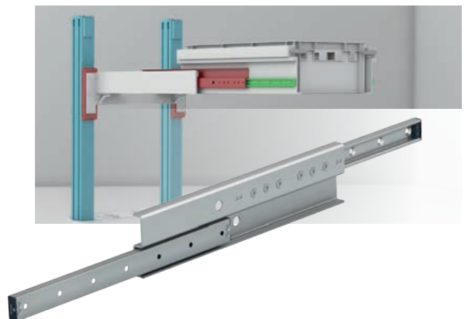
Telescopic totes grabber
