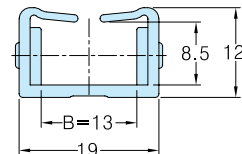
A-A Cross Section
