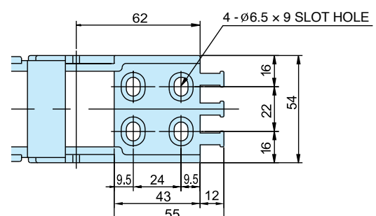
Moving Bracket
