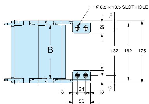
Moving Bracket
