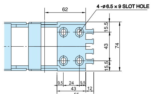
Moving Bracket
