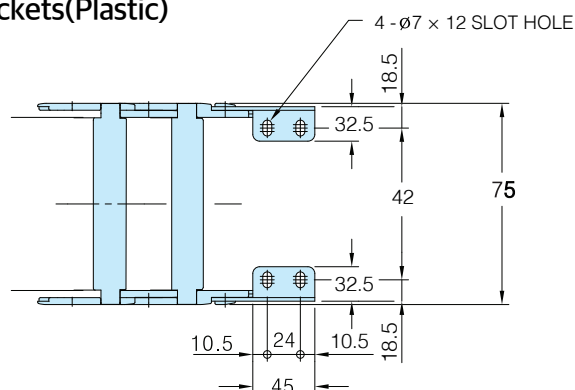
Fixed Bracket
