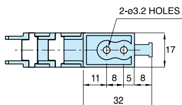
Fixed Bracket
