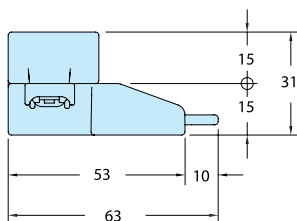
A TYPE
