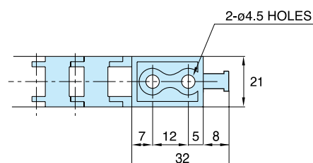
Moving Bracket
