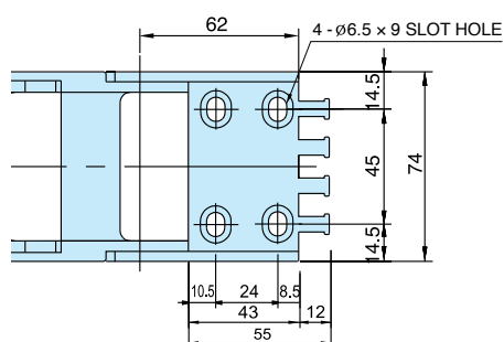
Fixed Bracket
