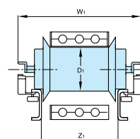
SECTION BB SUPPORT ROLLER
