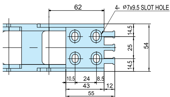
Fixed Bracket
