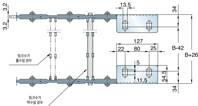
Fixed Bracket
