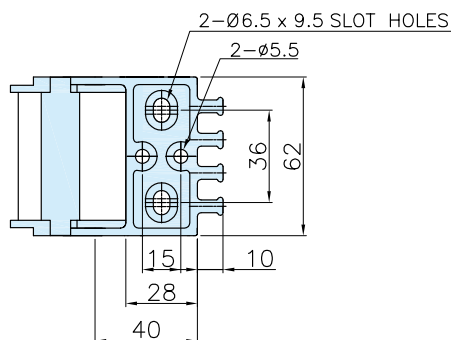
Fixed Bracket
