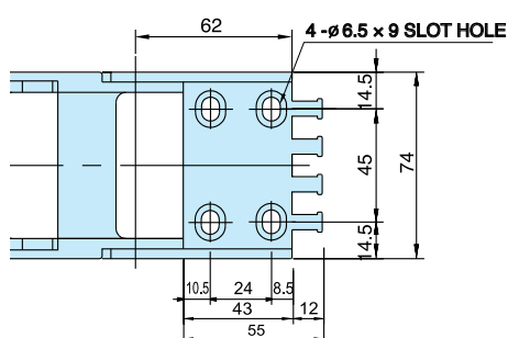
Fixed Bracket
