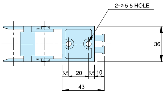
Fixed Bracket
