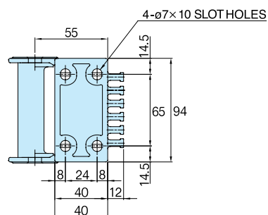
Fixed Bracket
