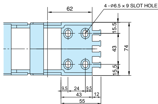
Moving Bracket
