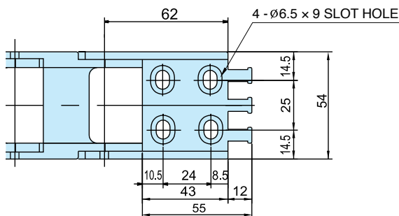
Fixed Bracket
