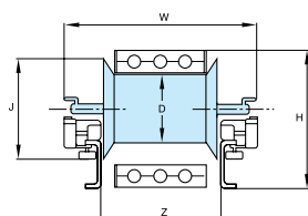
SECTION AA GUIDE ROLLER
