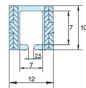
A-A Cross Section
