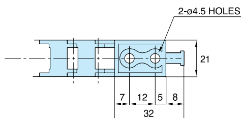
Fixed Bracket
