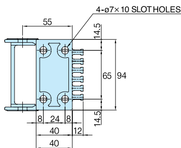
Fixed Bracket
