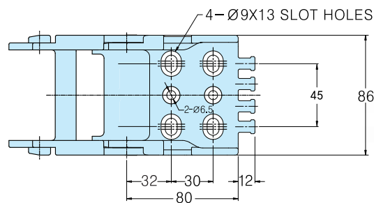
Moving Bracket
