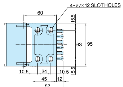
Moving Bracket
