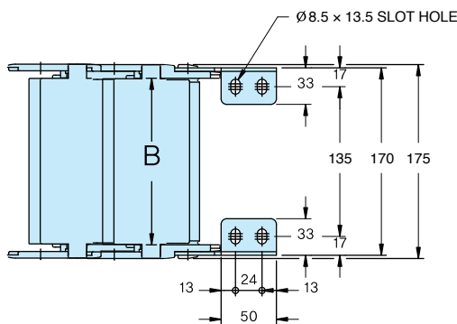
Fixed Bracket
