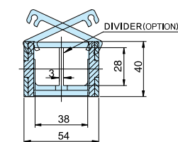
A-A Cross Section
