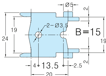
Moving-Fixed Link
