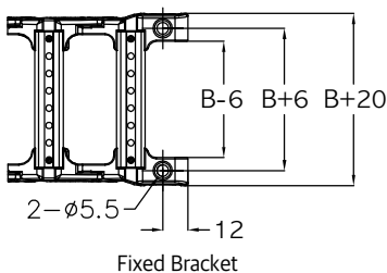
Fixed Bracket
