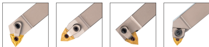
MWLN□95° MWMNN50° MWWN□50° WWLN□95°
