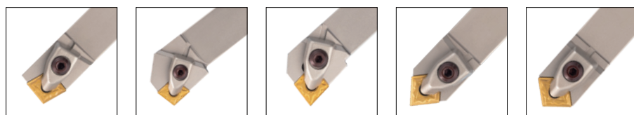
DCBN□75° DCKN□75° DCLN□95° DCMNN50° DCMNN-100 40°
