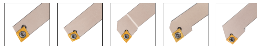
SCAC□90° SCBC□75° SCFC□91° SCGC□91° SCKC□75°
