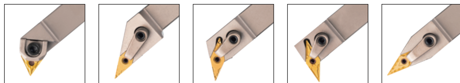
WTQN□105° MVJN□93° MVQN□117.5° MVUN□95° MVVNN72.5°
