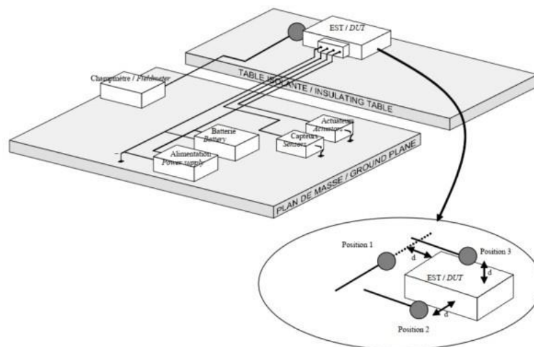
Figure 5. Test setup example for electrical components of a vehicle (source: PSA standard)
