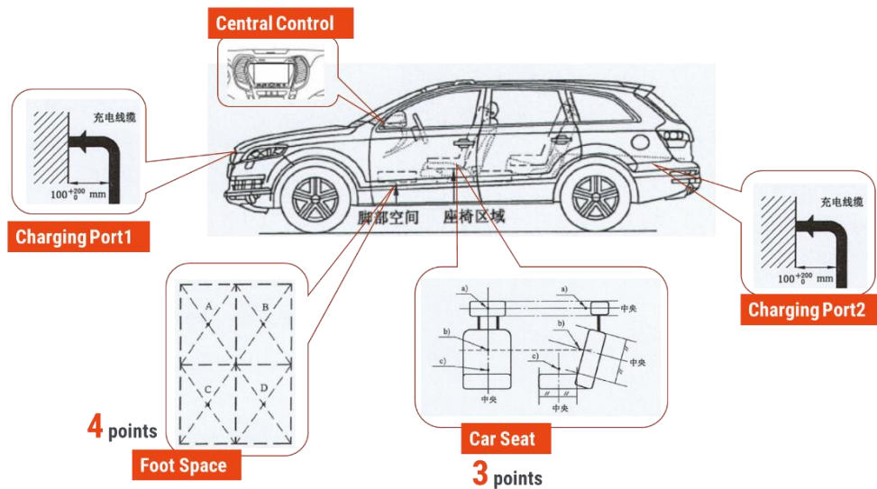
Figure 3. Electric vehicle test points
