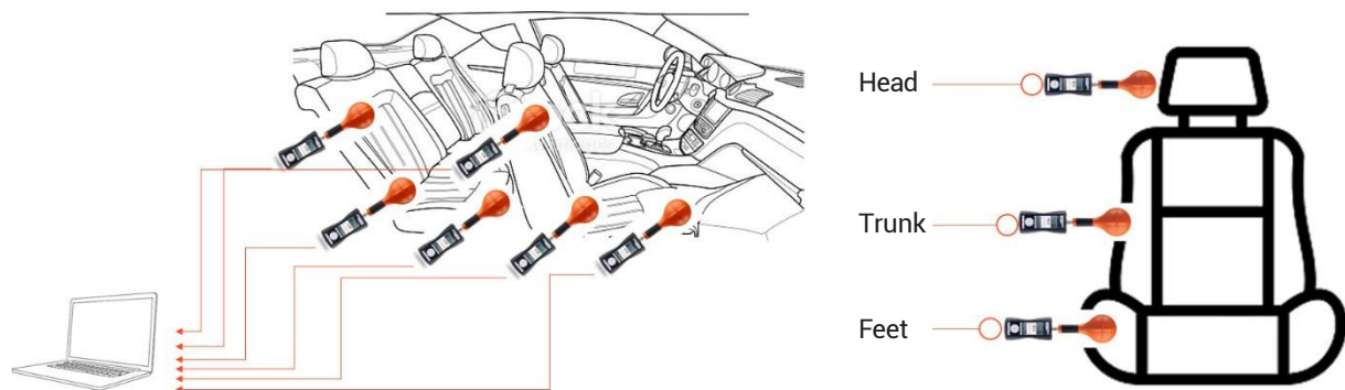
Figure 4. Seat points to be measured (Head, Trunk and Leg)
