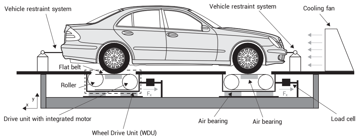
Figure 2. Picture of vehicle on a dynamometer during testing
