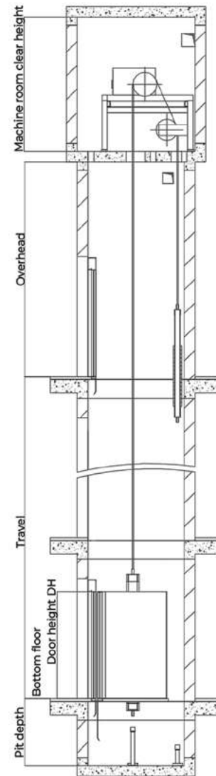
Hoistway section
