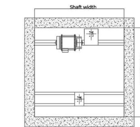
Overhead floor layout drawing
