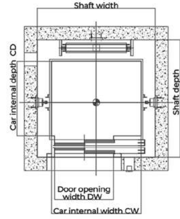
Shaft layout drawing
