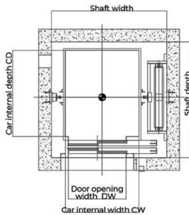
Shaft layout drawing
