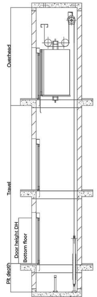
Hoistway section
