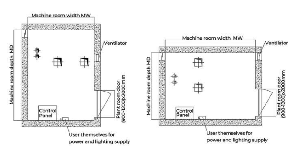
Machine room layout drawing
