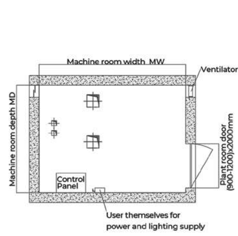
Machine room layout drawing
