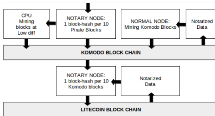
Figure 2: A block schematic representation of delayed Proof-of-Work.
