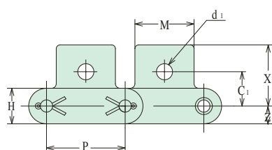
SK-1 attachment
