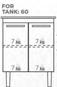
WASHING TANK CABINET W: 50 cm H: 91 cm D: 53,5 cm
