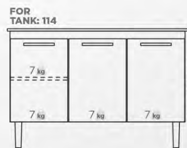
WASHING TANK CABINET W: 117 cm H: 91 cm D: 53,5 cm
