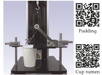
Container seal peeling test
