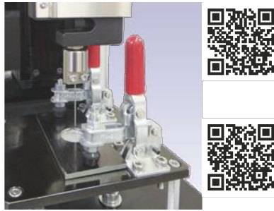
Food packaging puncture test
