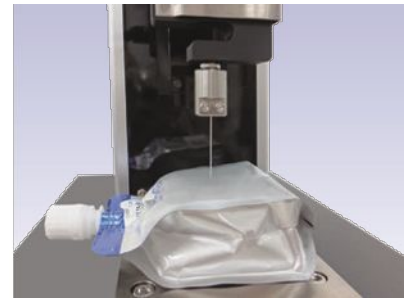
Packing container puncture resistance test
