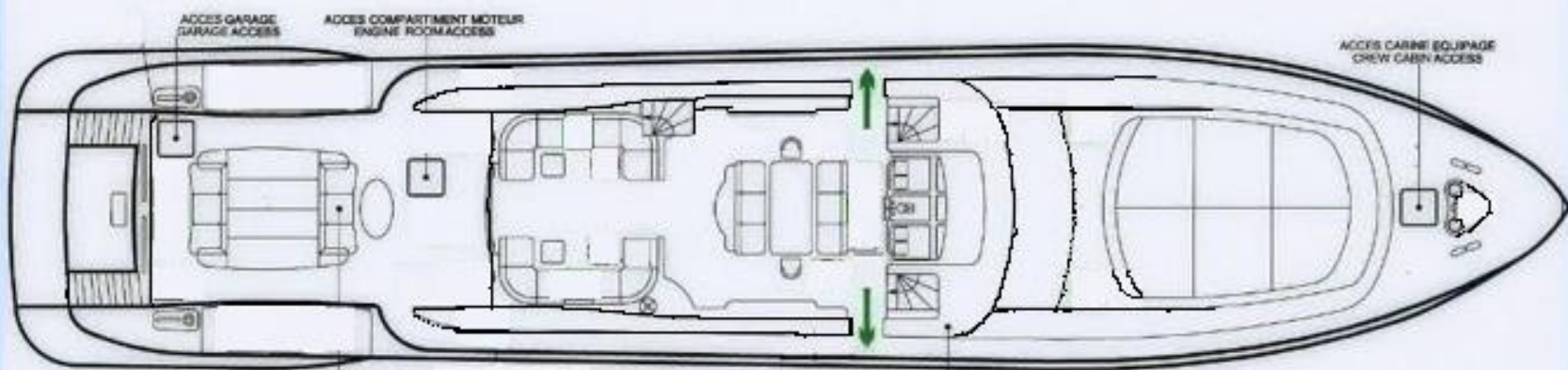
PONT PRINCIPAL / MAIN DECK
