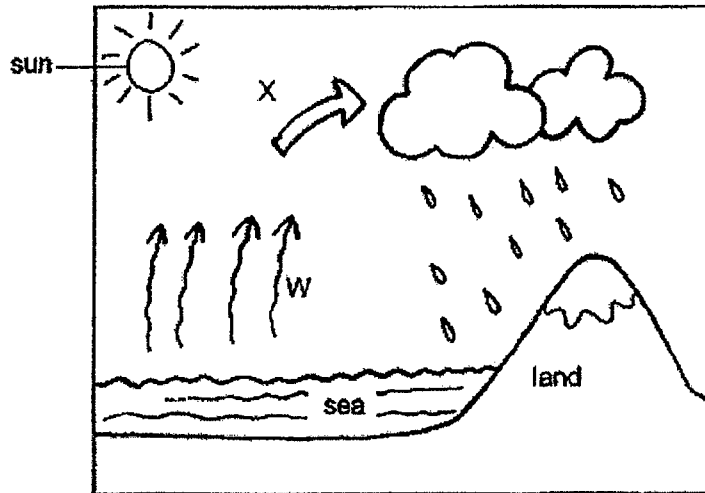
Water cycle
