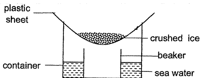
Set-up R
