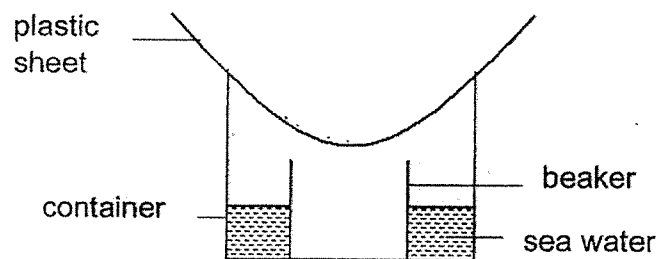
Set-up W
