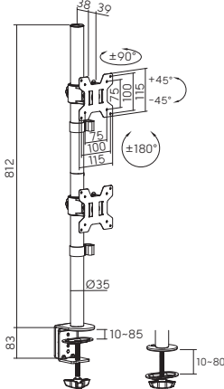
MP0292-17 Vertical Dual-Monitor; Clamp-on / Grommet
