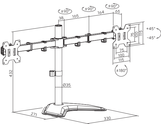
MP0292-09 Dual-Monitor; Freestanding Base
