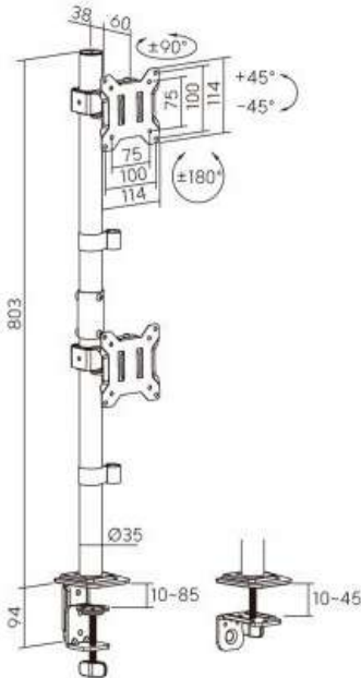
LDT110-C02V Clamp / Grommet
