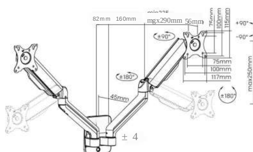
LDA32-114E For Dual Monitor
