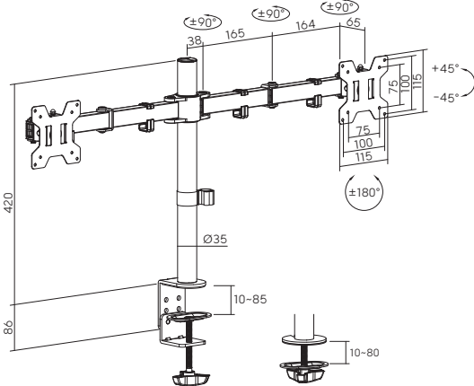
MP0292-17 Vertical Dual-Monitor; Clamp-on / Grommet
