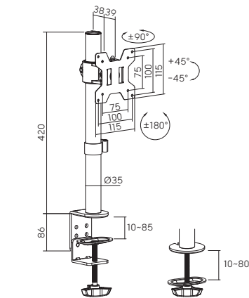
MP0292-14 Single-Monitor; Clamp-on / Grommet
