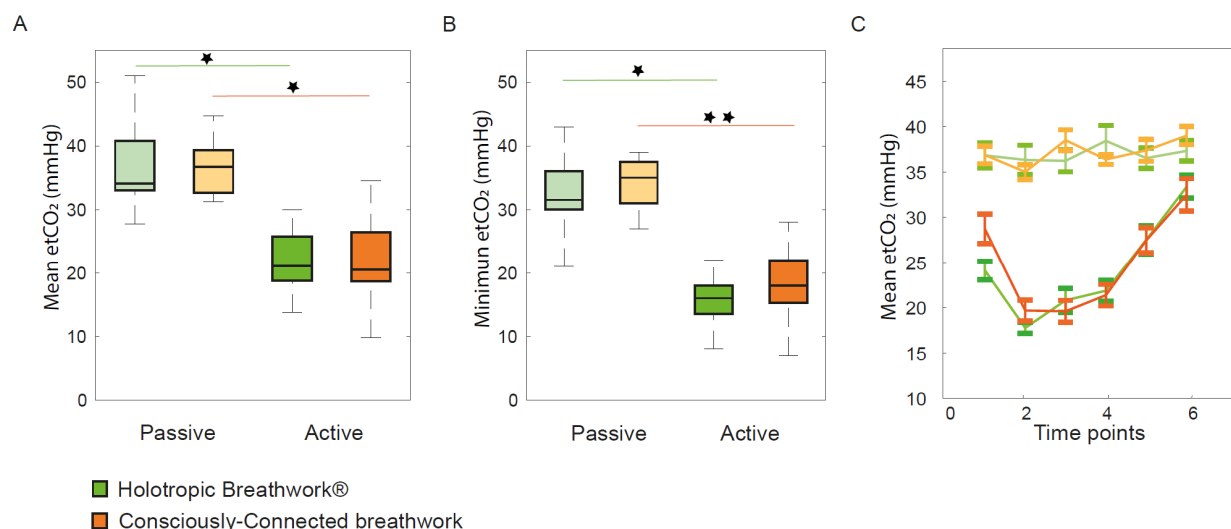
Figure 1. End-tidal CO 2 saturation during breathwork. (A) Boxplot of mean partial end-tidal CO 2 pressure (etCO 2 ) per subject, pooled across the active portion of the breathwork session (time points 2-4 out of 6). Central line: Median. Box outline: 25 th and 75 th percentile. Whiskers: 10 th and 90 th percentile. Green: Holotropic Breathwork®. Orange: Consciously-Connected breathwork. Desaturated colours (on the left): Passive-breath control groups. Saturated colours (on the right): Active-breath groups. Both active-breath groups showed significantly lower etCO 2 than their passive-breath counterparts. (B) Same as A for minimum etCO 2 per subject across measurement time points 2-4. Differences between active and passive breath groups are even more pronounced, with active-breath participants reaching etCO 2 as low as 10-20 mmHg throughout the session. (C) Time course of etCO 2 across all six measurement time points. etCO 2 decreased rapidly at the start of the session, reaching their minimum around measurement time points 2-3, and then increasing gradually towards the end of the session.
