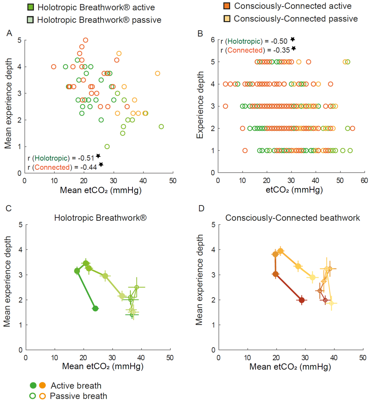
Figure 3. Relationship between end-tidal CO 2 saturation and experience depth. (A) Scatter plot showing mean experience depth per subject, averaged across measurement time points 2-4, as a function of mean end-tidal CO 2 pressure (etCO 2 ) averaged across the same interval. Colour scheme as in Figures 1 and 2. Mean etCO 2 and experience depth were negatively correlated for both Holotropic Breathwork® and Consciously-Connected breathwork, indicating that lower etCO 2 levels throughout the session were associated with deeper altered states of consciousness. (B) Same as A, but for six raw, i.e. non-averaged, measurements of etCO 2 and experience depth per subject. etCO 2 and experience depth were again negatively correlated. (C) Average trajectory
