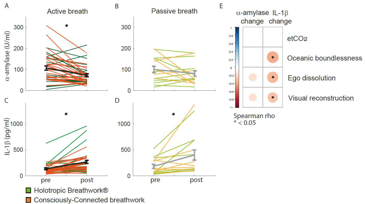
Figure 5. Subacute physiological effects of breathwork. (A) Concentration of the autonomic nervous system activity marker alpha-amylase ( \alpha -amylase) directly before and after the breathwork session, completed by a total of 39 participants in the active-breath group. Orange lines: Participants in Consciously-Connected breathwork. Green lines: Participants in Holotropic Breathwork®. Black line and error bars: Mean \pm SEM across participants. Star indicates statistically significant decrease in \alpha -amylase at an Alpha level of 0.05. (B) Same as A for passive-breath participants (n=15). Light orange: Consciously-Connected breathwork. Light green: Holotropic Breathwork®. Grey line and error bars: Mean \pm SEM. (C) Same as A for concentrations of the inflammatory marker interleukin-1 beta (IL-1 \beta ). Star indicates statistically significant increase in IL-1 \beta at an Alpha level of 0.05. (D) Same as B for concentrations of IL-1 \beta . Star indicates statistically significant increase in IL-1 \beta at an Alpha level of 0.05. (E) Same as Figure 4E for correlations between the acute aspects of the breathwork session and the post-breathwork changes in \alpha -amylase and IL-1 \beta levels. IL-1 \beta increases were linked to subjective experiences, but not etCO 2 , during breathwork, such that deeper ASCs predicted smaller increases in IL-1 \beta post-session. Change in \alpha -amylase was not significantly predicted by any of the acute parameters of the breathwork session.
