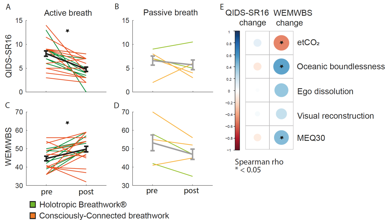
Figure 4. Psychological effects of breathwork. (A) Scores of the Self-Report Quick Inventory of Depressive Symptomatology (QIDS-SR16) one week before and after the breathwork session, completed by a total of 27 participants in the active-breath group. Orange lines: Participants in Consciously-Connected breathwork. Green lines: Participants in Holotropic Breathwork®. Black line and error bars: Mean \pm SEM across participants. Star indicates statistically significant decrease in QIDS-SR16 scores at an Alpha level of 0.05. (B) Same as A for the passive-breath group that completed follow-on questionnaires (n=5). Light orange: Consciously-Connected breathwork. Light green: Holotropic Breathwork®. Grey line and error bars: Mean \pm SEM. (C) Same as A for scores in the Warwick-Edinburgh Mental Wellbeing Scale (WEMWBS). Star indicates statistically significant increase in WEMWBS scores at an Alpha level of 0.05. (D) Same as B for WEMWBS scores. (E) Correlations between post-breathwork changes in QIDS-SR16 and WEMWBS scores on the one hand, and acute aspects of the breathwork session on the other hand, specifically average etCO 2 during the active part of the session, as well as scores in the Mystical Experiences Questionnaire 30 (MEQ30) and the three subscales of the 11-Dimensional Altered States of Consciousness scale (11-DASC), which are termed 'Oceanic boundlessness', 'Ego dissolution' and 'Visual reconstruction'. Correlation strength is colour-coded (see in-figure legend). Stars indicate statistically significant correlations. Correlations were computed based on 32 participants who completed questionnaires at the 1-week follow-up of the breathwork session. Post-breathwork changes in QIDS-SR16 scores were not significantly predicted by any of the acute parameters of the breathwork session. In contrast, improvements in WEMWBS scores were predicted by lower etCO 2 and by deeper ASCs during the session, indicated by both MEQ30 and 11-DASC scores.
