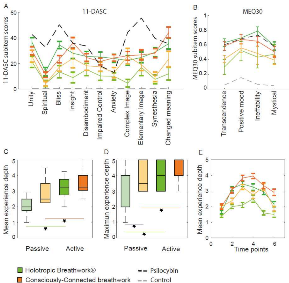
Figure 2. Experience depth during breathwork. (A) Subjective experience triggered by breathwork, as assessed by the 11-Dimensional Altered States of Consciousness Scale (11-DASC). Error bars: SEM. Colour scheme is the same as in Figure 1, with saturated colours denoting active-breath groups and desaturated colours denoting the passive-breath control groups. Black dashed line: Typical 11-DASC scores for a dose of 20-25mg Psilocybin, pooled across five relevant clinical studies of psilocybin-augmented therapy extracted from the Altered States of Consciousness Database (see Methods). Grey dashed lines: Typical 11-DASC scores for placebo treatments in three clinical studies extracted from the same data base. (B) Same as A for the four subscales of the Mystical Experiences Questionnaire 30 (MEQ30). Black dashed lines: Typical MEQ30 scores for a dose of 20-25mg Psilocybin, pooled across four relevant clinical studies from the Altered States of Consciousness Database (see Methods). Grey dashed lines: Same for placebo
