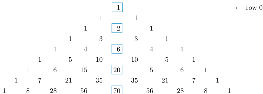
Figure 1.33 Pascal's Triangle.
