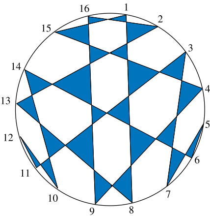
The (17, 8) residue design
