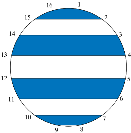
The (17, 16) residue design
