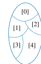
The set \mathbf{Z} of integers
