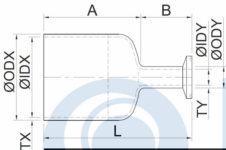
Tri - Clamp Weld, Cup for Drainage - JB 16WMP
