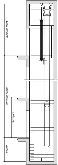
Machine roomless passenger specifications
