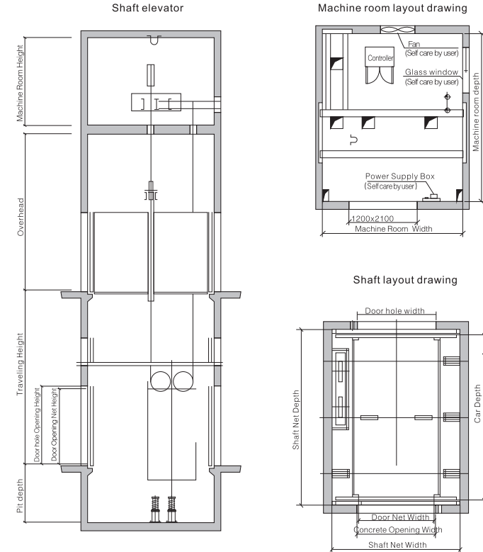
Car elevator specifications
