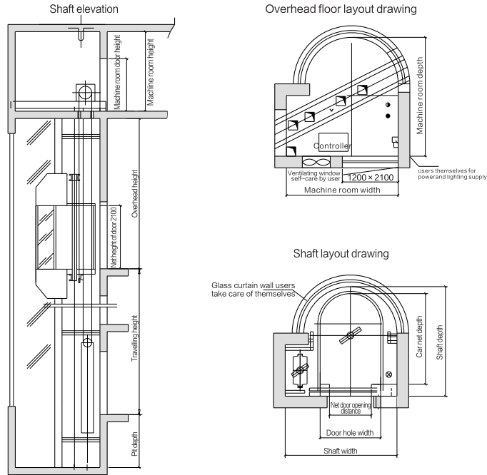
Semicircle machine room / Machine roomless elevator specifications
