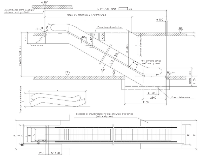
35° Escalator construction layout drawing
