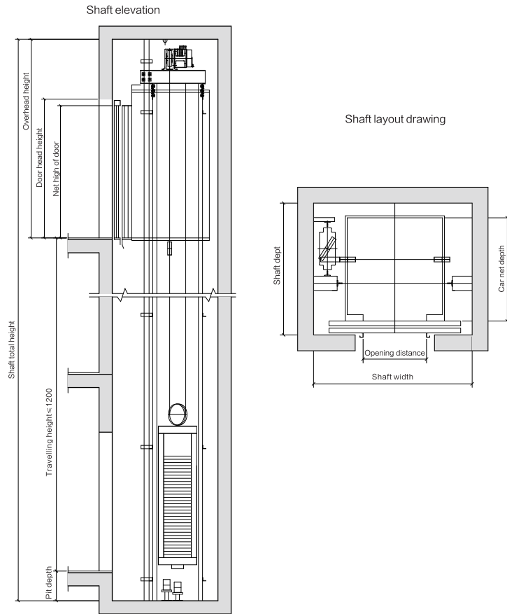
Villa elevator specifications
