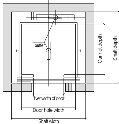
Shaft layout drawing
