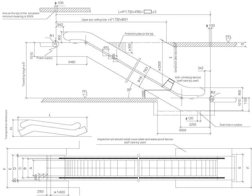
30° Escalator construction layout drawing
