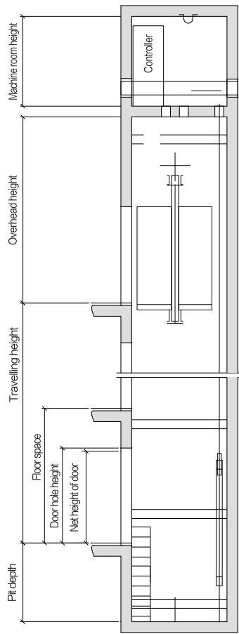
Shaft elevation
