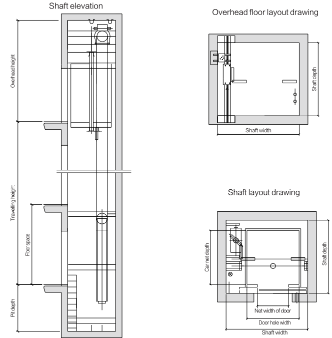
Square machine room / Machine roomless elevator specifications
