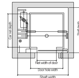
Shaft layout drawing
