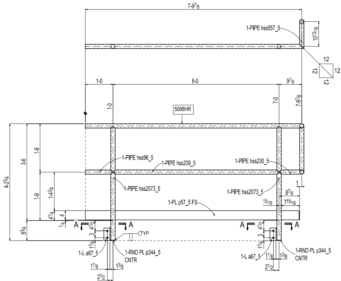
ONE HANDRAIL 5068HR
