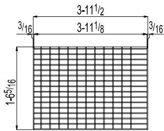
ONE GRATING 230G6
