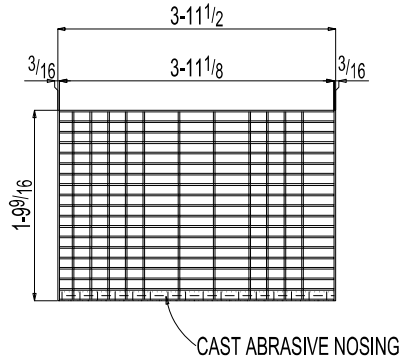
ONE GRATING 230G5
