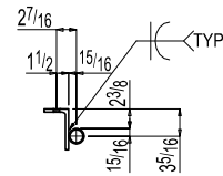
Section A-A 5068HR
