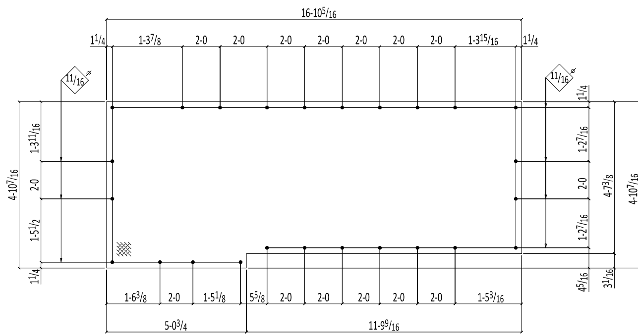
ONE CHECKERED PLATE 130M2
