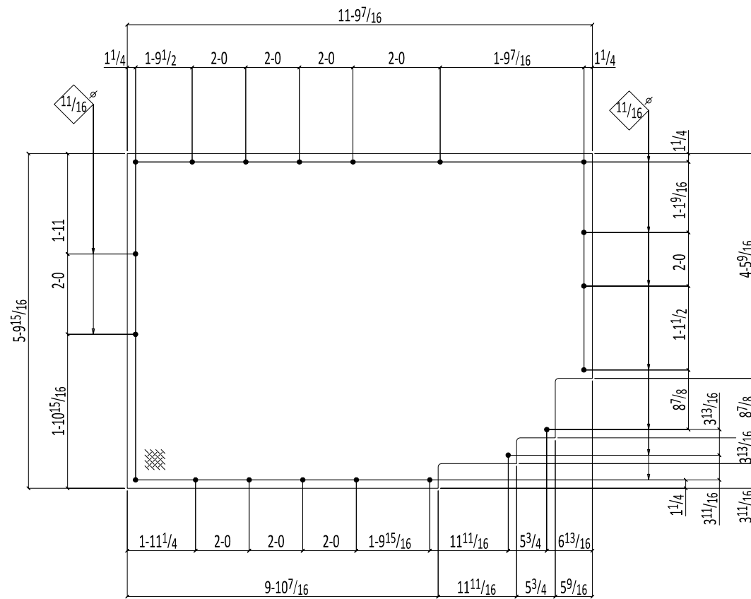
ONE CHECKERED PLATE 130M3
