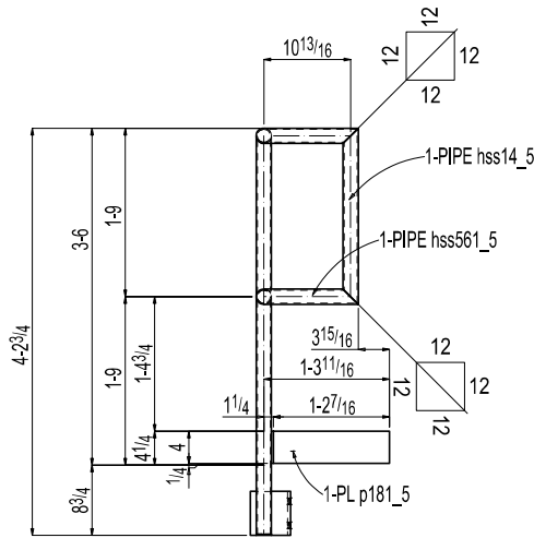
Section A-A 5068HR
