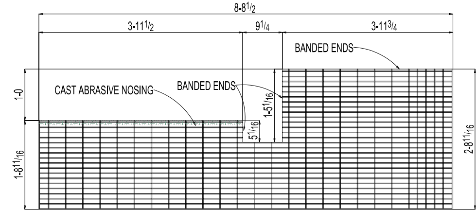
ONE GRATING 230G3
