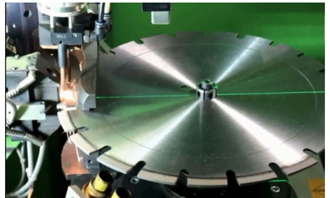
Prime Diamond Saw Blade Laser Welding in progress
