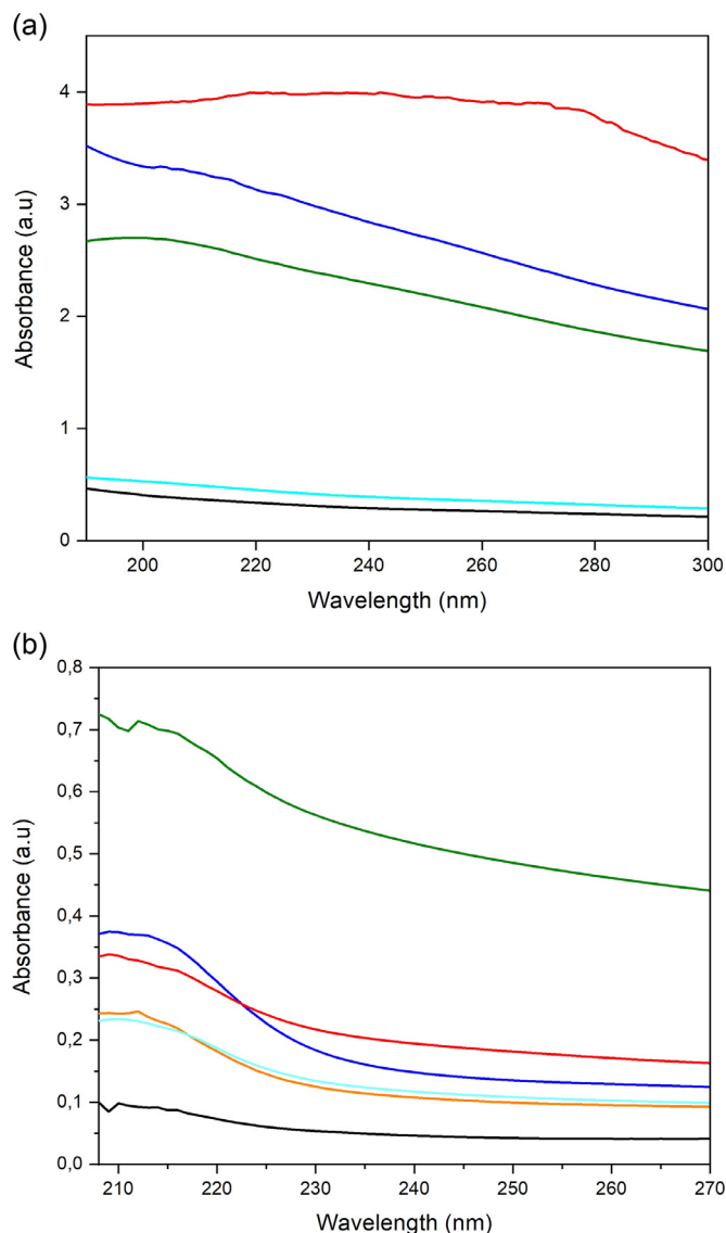
Fig. 8. Stability assays a) in bidistilled water and b) real water sample.
