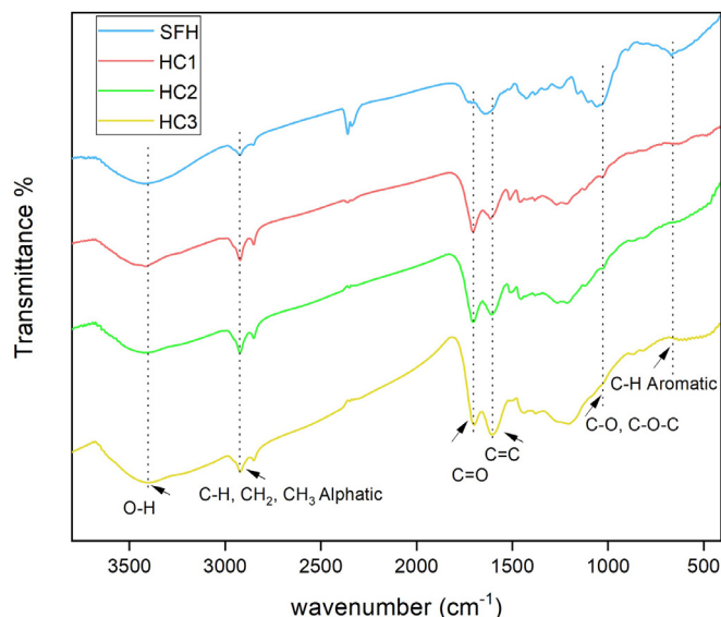
Fig. 1. FTIR spectra of SFH and HC.
