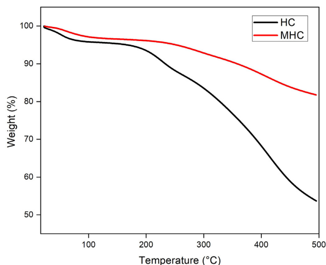
Fig. 7. Weight loss as function of temperature for MHC and HC.
