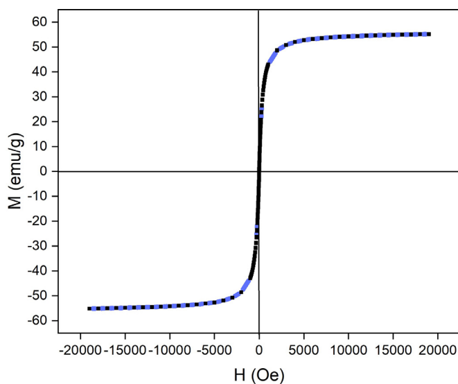
Fig. 5. Magnetization curve at room temperature for MHC.
