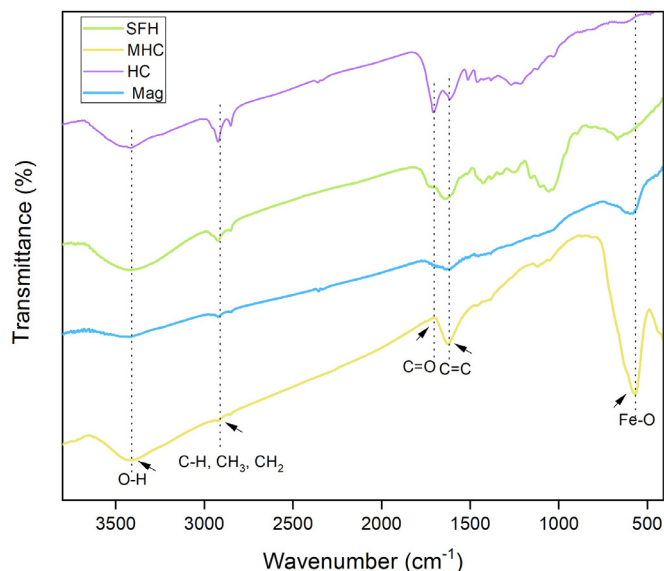
Fig. 2. FTIR spectra of HC and MHC.
