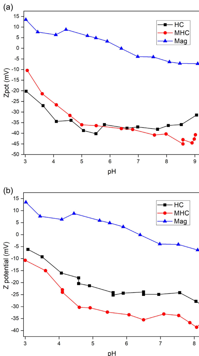
Fig. 6. Z potential as function of pH of HC, MHC and naked magnetite in different electrolytes: a) 0.001 M \text{KNO}_3 (HC and MHC initial pH :4.79 and 6.41), b) 0.001 M NaCl (HC and MHC initial pH :5.55 and 5.36).
