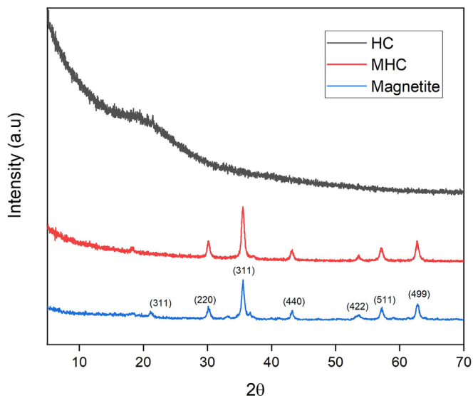
Fig. 3. X-ray diffraction patterns of MHC and HC.
