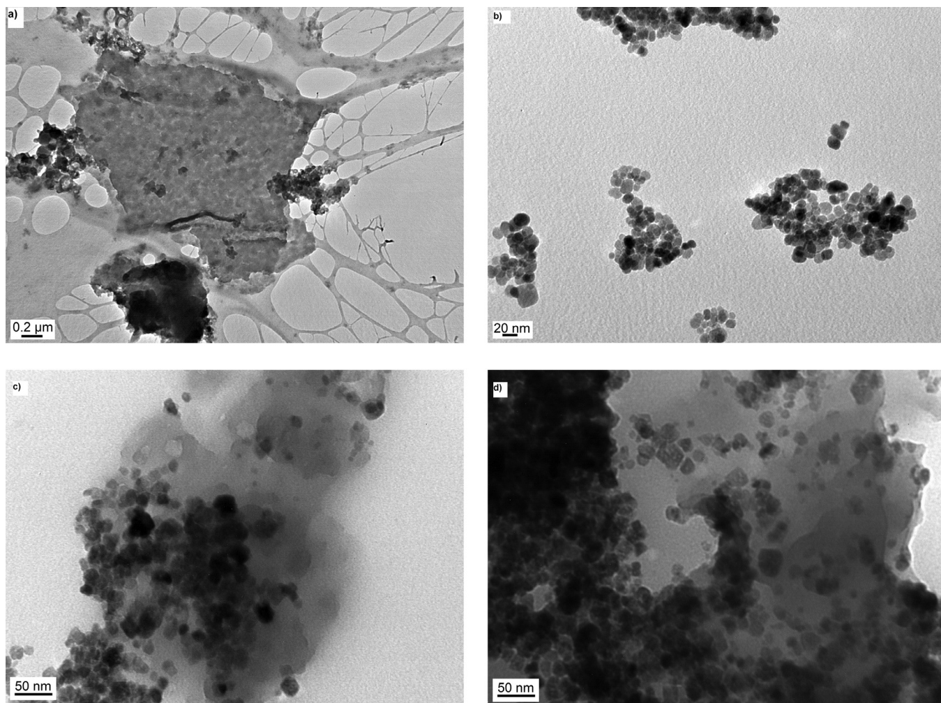
Fig. 4. TEM images of a) HC, b) neck magnetite, c and d) MHC.
