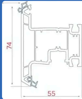
AST - 551 - S01 OUTWARD OPENING WINDOW SASH / T-MULLION
