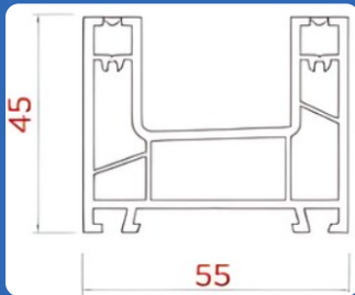
AST - 550 - F01 2 TRACK OUTER FRAME
