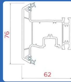
AST - 621 - SO2 OUTWARD OPENING WINDOWS SASH / T MULLION
