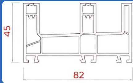
AST - 550 - F02 2.5 TRACK OUTER FRAME
