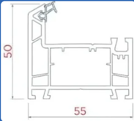
AST - 551 - F01 WINDOW OUTER FRAME
