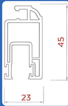
AST - 550 - M01 WINDOW BUG SCREEN SASH
