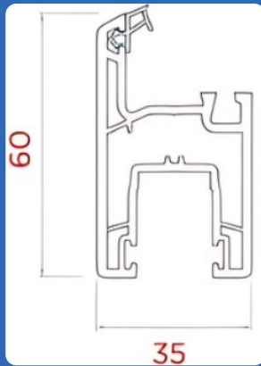
AST - 550 - S01 WINDOW SASH
