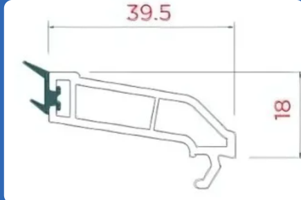
AST 181 - BO1 GLAZING BEAD :- 40MM
