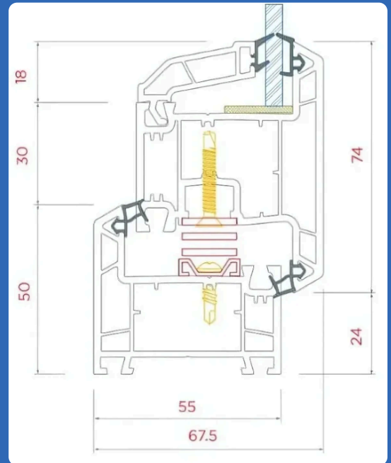
AST - 551 - S01 OUTWARD OPENING WINDOW SASH / T-MULLION
