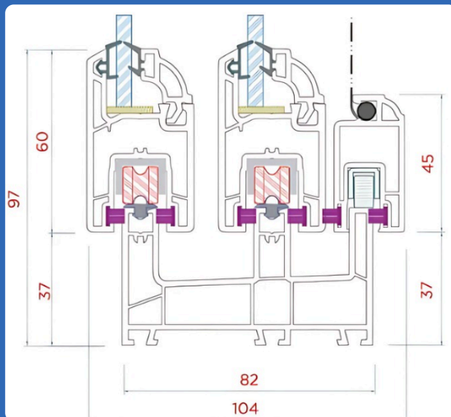
AST - 550 - S01 WINDOW SASH
