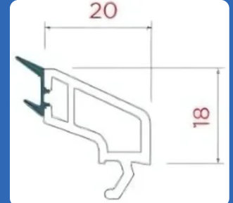
AST 181 - BO4 GLAZING BEAD :- 20MM
