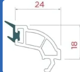
AST 181 - BO3 GLAZING BEAD :- 24MM
