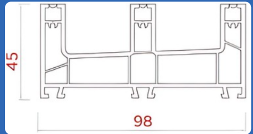
AST - 550 - F03 3 TRACK OUTER FRAME
