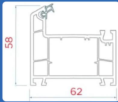
AST - 621 - FO1 WINDOW OUTER FRAME
