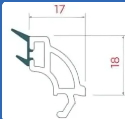
AST 181 - BO5 GLAZING BEAD :- 17MM
