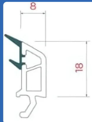
AST 181 - BO6 GLAZING BEAD :- 8MM
