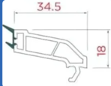
AST 181 - BO2 GLAZING BEAD :- 35MM
