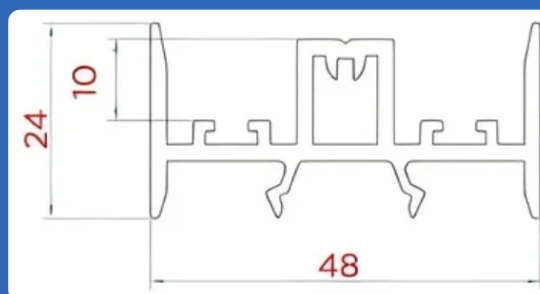
AST - 620 - AO1 INLINE SASH ADAPTER
