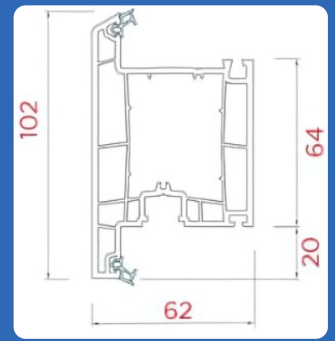
AST - 621 - SO2 OUTWARD OPENING DOOR SASH
