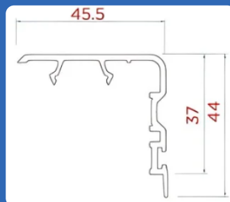
AST - 620 - LINTERLOCK FOR WINDWO SASH
