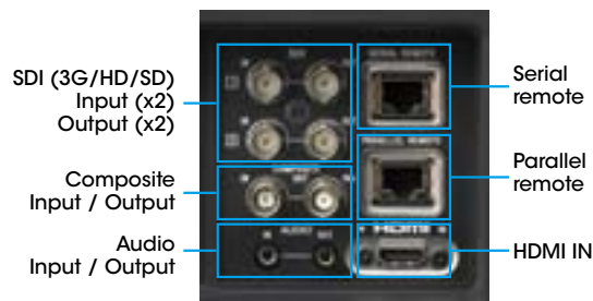
PVM-A250 rear
