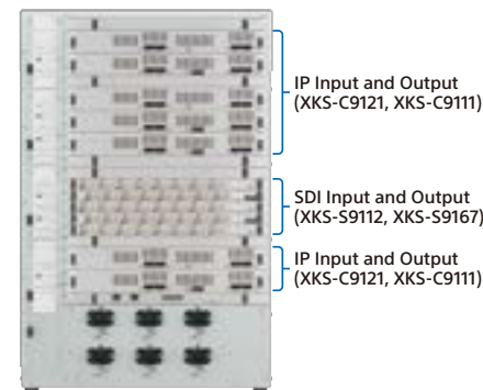
XVS-9000 (Rear)
