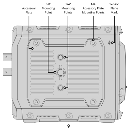
2 x 3/8" and 7 x 1/4" Tripod Mounting Points
