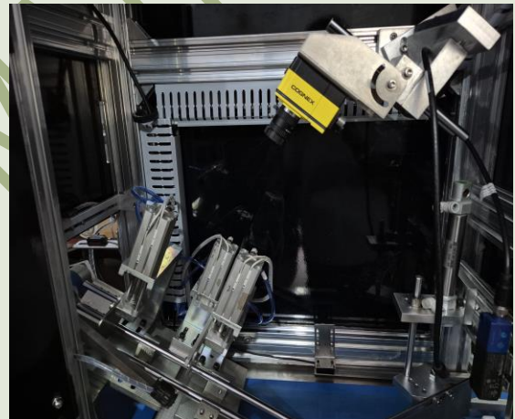
BEARING LENGTH CHECKING MACHINE
