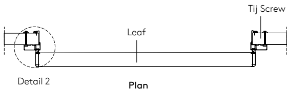
Plan
