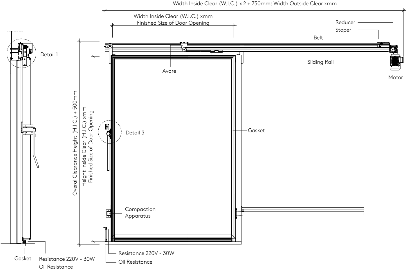
Front Elevation
