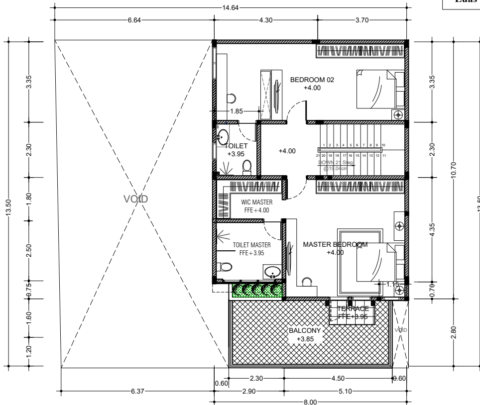
DENAH LT. 2 SKALA 1: 100
