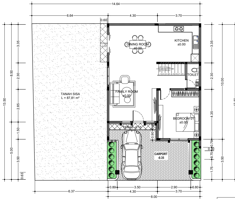
DENAH LT. 1 SKALA 1: 100
