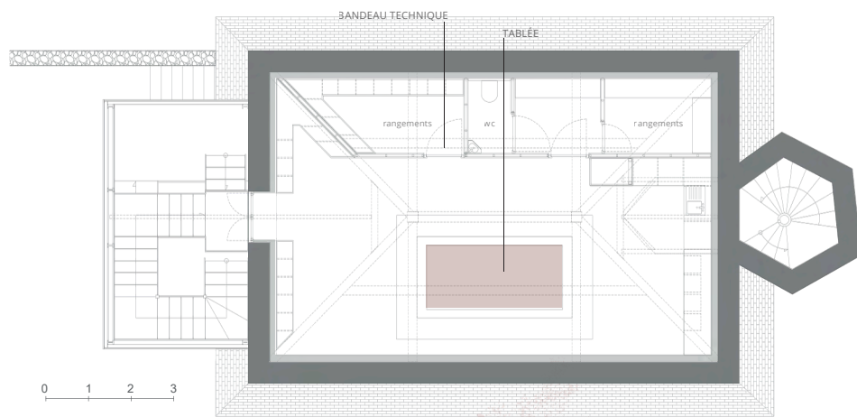
PLAN COMBLES
