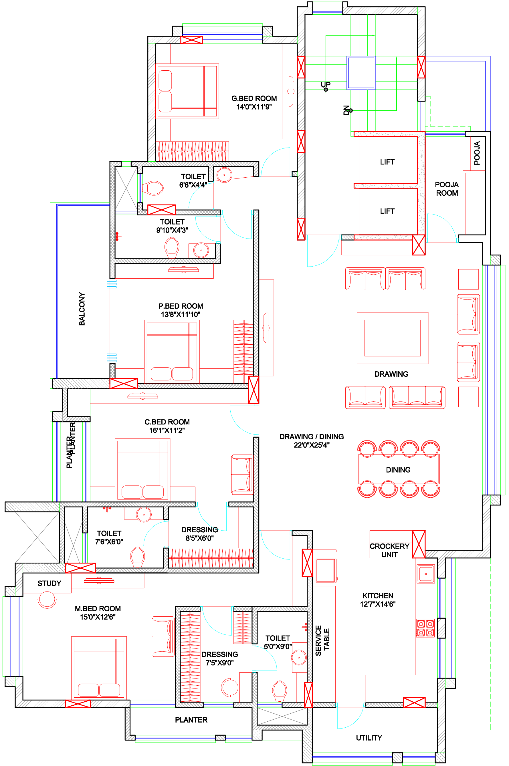
TYPICAL 6, 7th FLOOR PLAN
