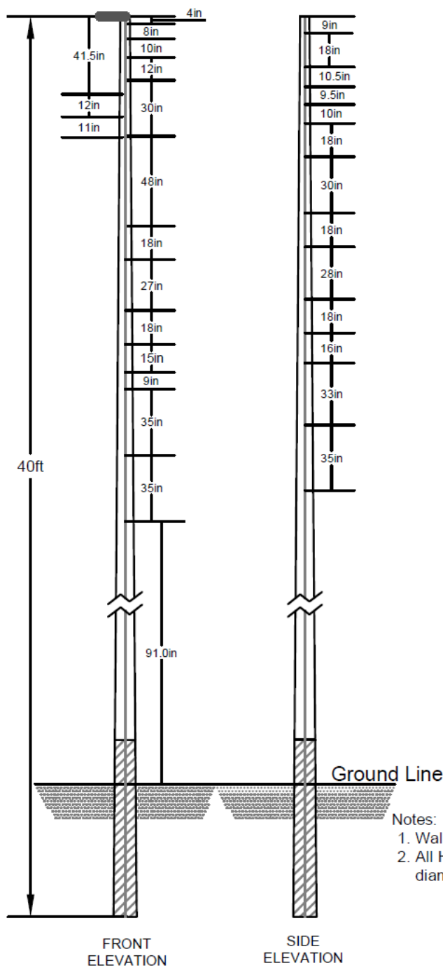
40FT STEEL POLE HOLE DETAILS
