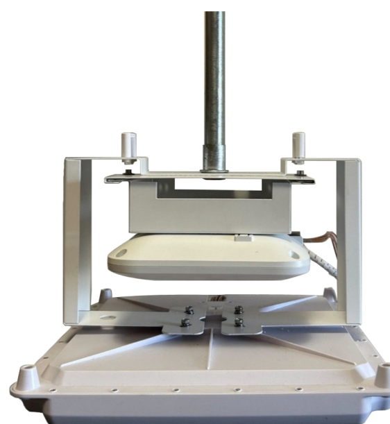
Antenna Mount with AP Drop Mount (Type B)
