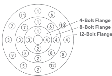
Flange Bolt Tightening Patterns
