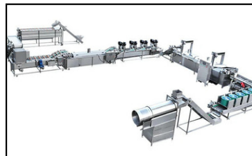
14) Potato Chips Plant
