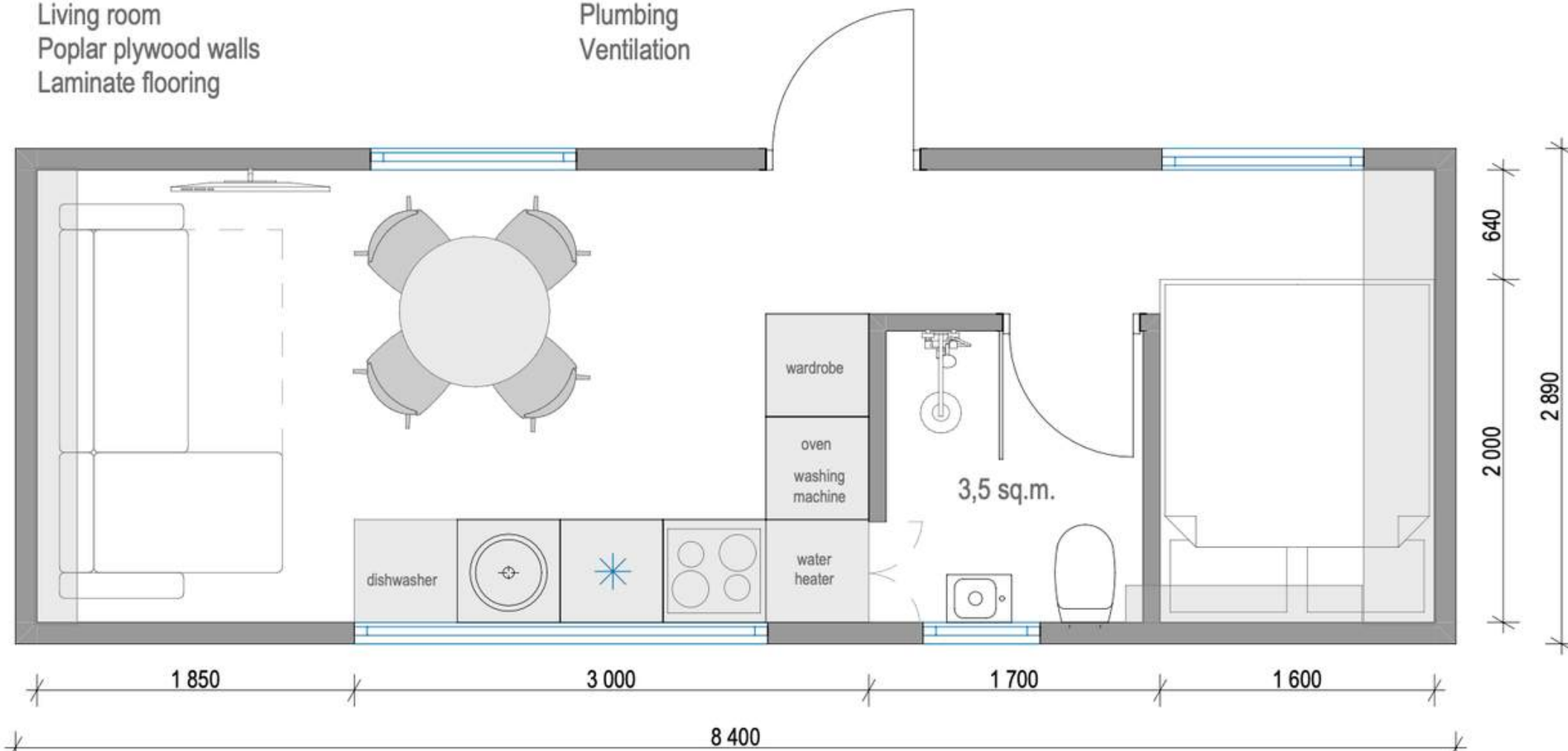
TINY HOUSE - MAXI 24 sq.m.
