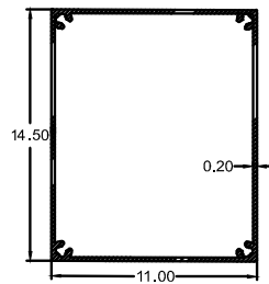
PILLAR PROFILE
