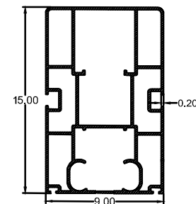
RAIL PROFILE
