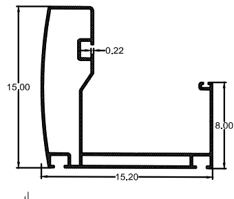
GUTTER PROFILE
