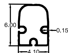
FABRIC SUPPORT PROFILE
