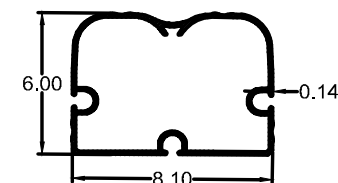
FABRIC CARRIER PROFILE
