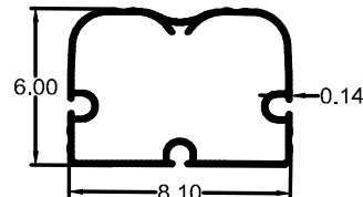
FABRIC CARRIER PROFILE
