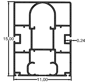
RAIL PROFILE
