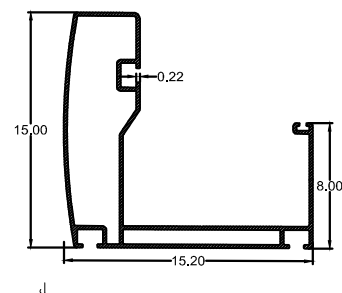
GUTTER PROFILE
