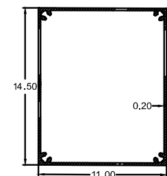
PILLAR PROFILE
