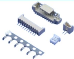
1.25mm Pitch Connectors
