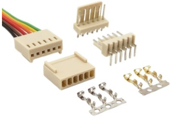
2.54mm Pitch Relimate Connectors
