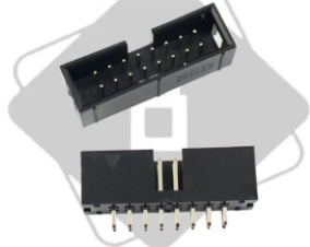
Shrouded Male Header - 2x8 - 2.54mm Pitch - 16 pin IDC connector - Straight
