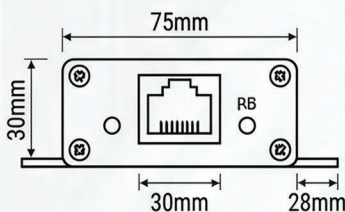
RJ45 Port
