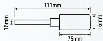
Temperature & Humidity Sensor
