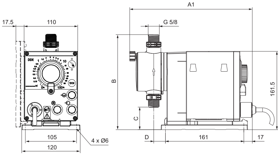
Fig. 3 Plano dimensional
