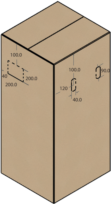
ISOMETRIC VIEW (EXTERNAL DIMENSIONS)
