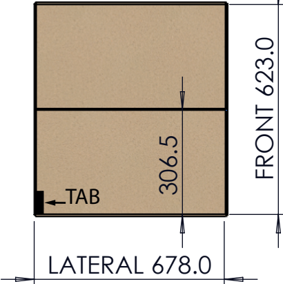
UPPER VIEW (INTERNAL DIMENSIONS)
