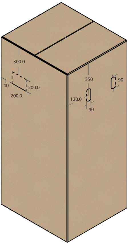
ISOMETRIC VIEW (EXTERNAL DIMENSIONS)
