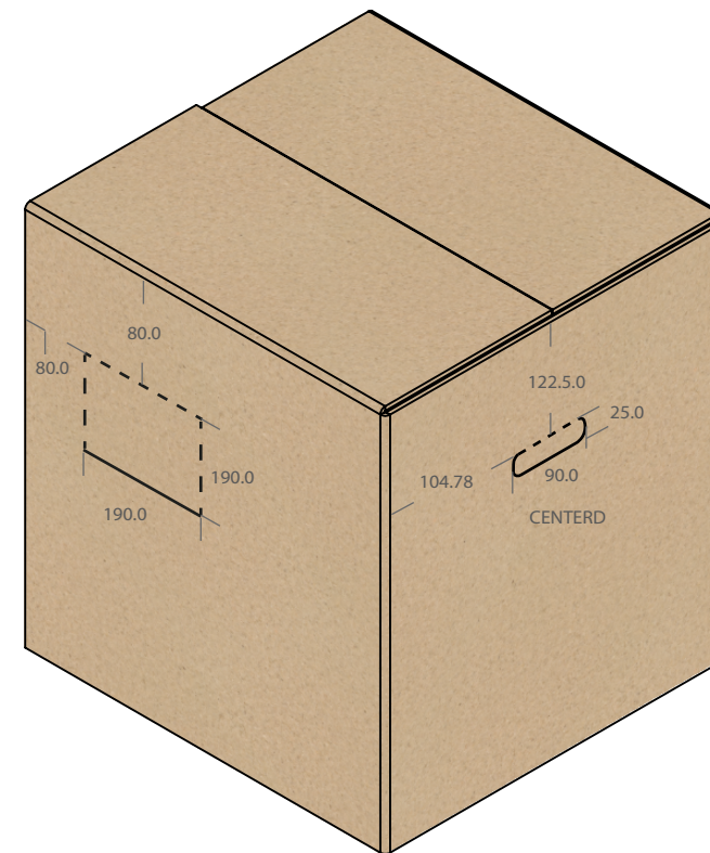
ISOMETRIC EXTERNAL VIEW (EXTERNAL DIMENSIONS)
