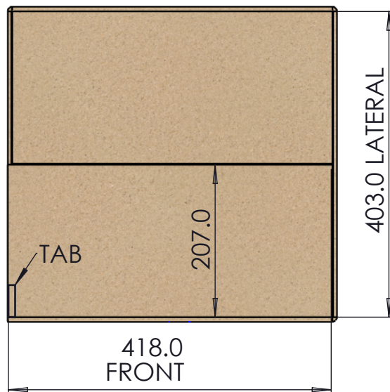
UPPER VIEW (INTERNAL DIMENSIONS)
