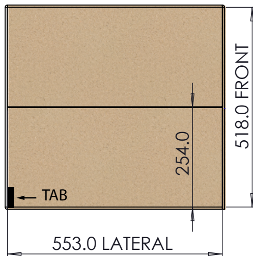
UPPER VIEW (INTERNAL DIMENSIONS)
