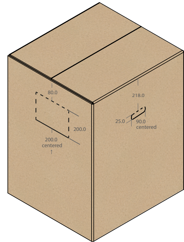
ISOMETRIC VIEW (EXTERNAL DIMENSIONS)
